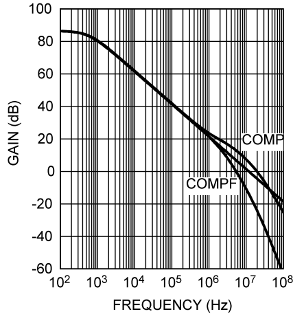
Figure 37. Transconductance Amplifier Open Loop Gain Figure 38. Transconductance Amplifier Open Loop Phase
