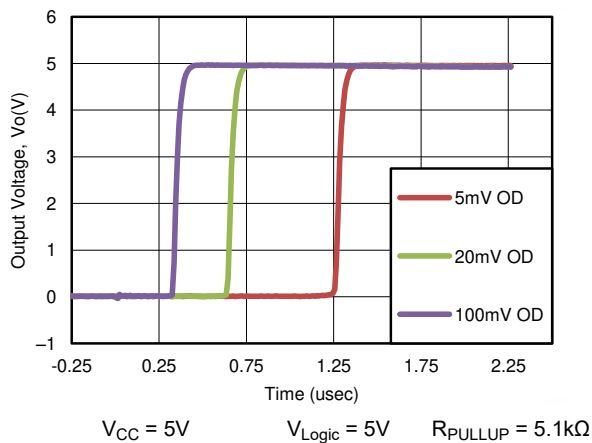
Figure 8-2. Response Time vs Output Voltage (Positive Transition)
