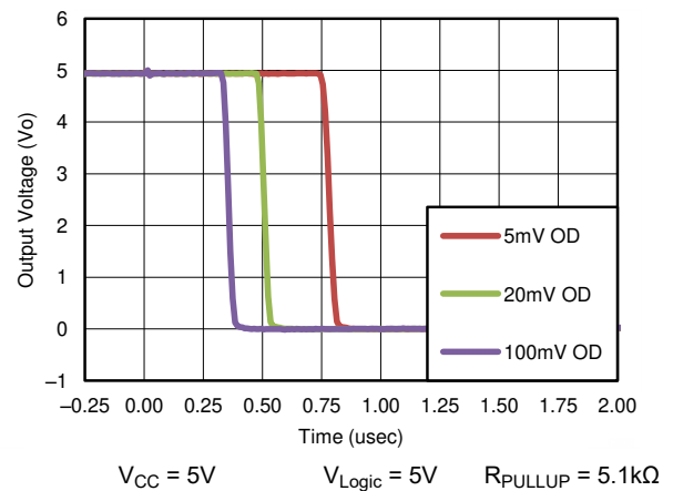
Figure 8-3. Response Time vs Output Voltage (Negative Transition)
