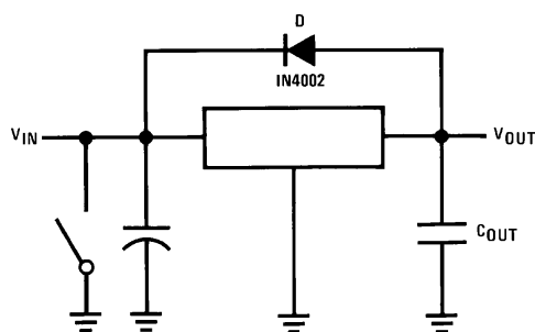
Figure 15. Input Short
