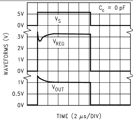
Figure 7. Response Time for 3.3-V Version ( C_C = 0 pF)
