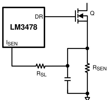
Figure 6-4. Adding External Slope Compensation
