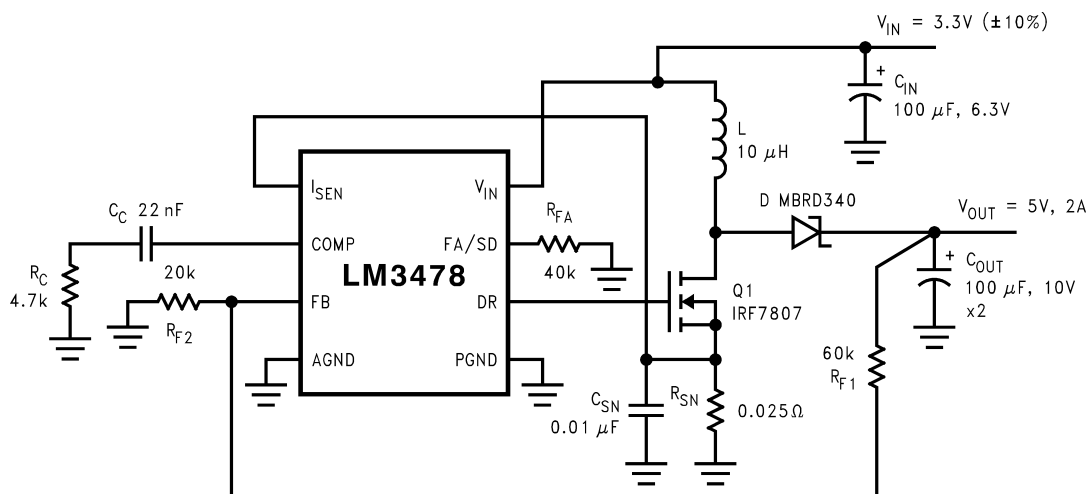
Figure 7-1. Typical High Efficiency Step-Up (Boost) Converter Schematic
