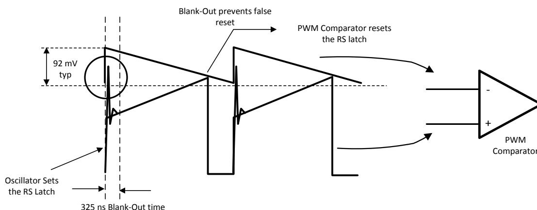
Figure 6-1. Basic Operation of the PWM Comparator
