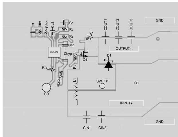
Figure 7-12. Typical Layout for a Boost Converter
