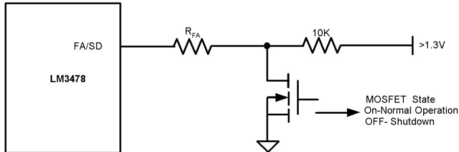
Figure 6-7. Shutdown Operation in Frequency Adjust Mode
