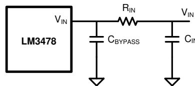
Figure 7-5. Reducing IC Input Noise
