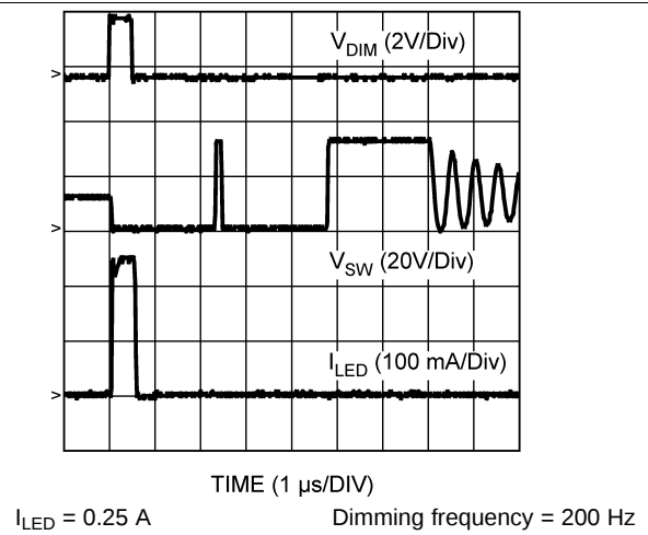
Figure 14. 10000:1 LED Dimming Waveforms
