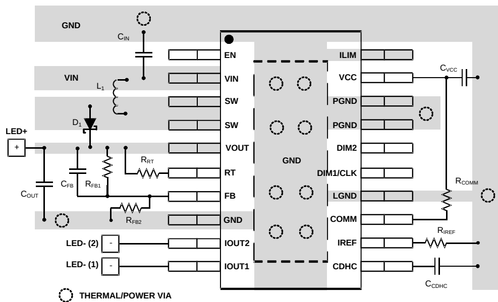
Figure 32. Layout Recommendation
