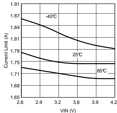
Figure 20. Closed Loop Current Limit vs V_{IN}
