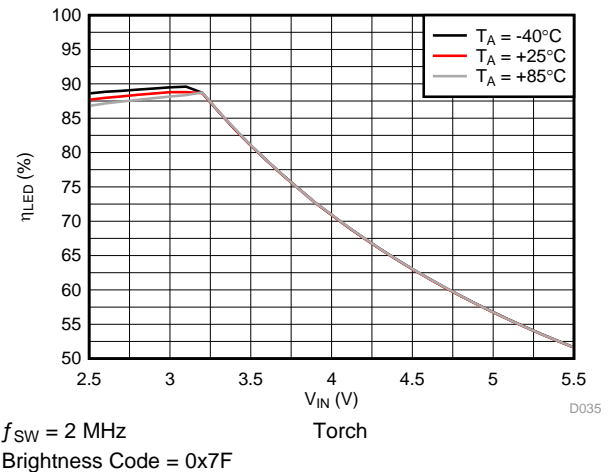
Figure 39. LED Efficiency vs Input Voltage
