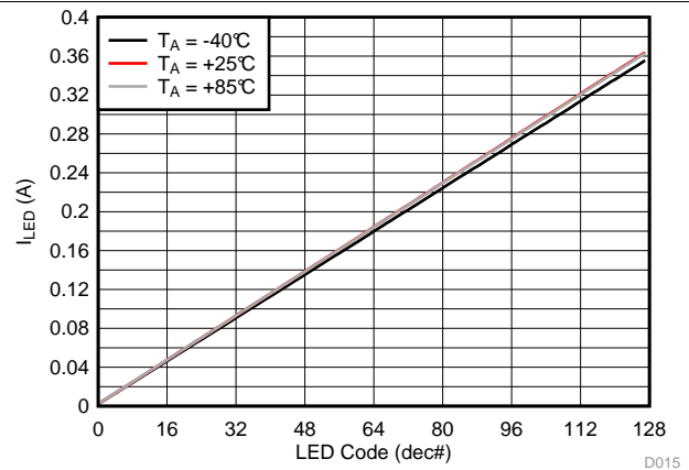
Figure 3. LED Torch Current vs Brightness Code
