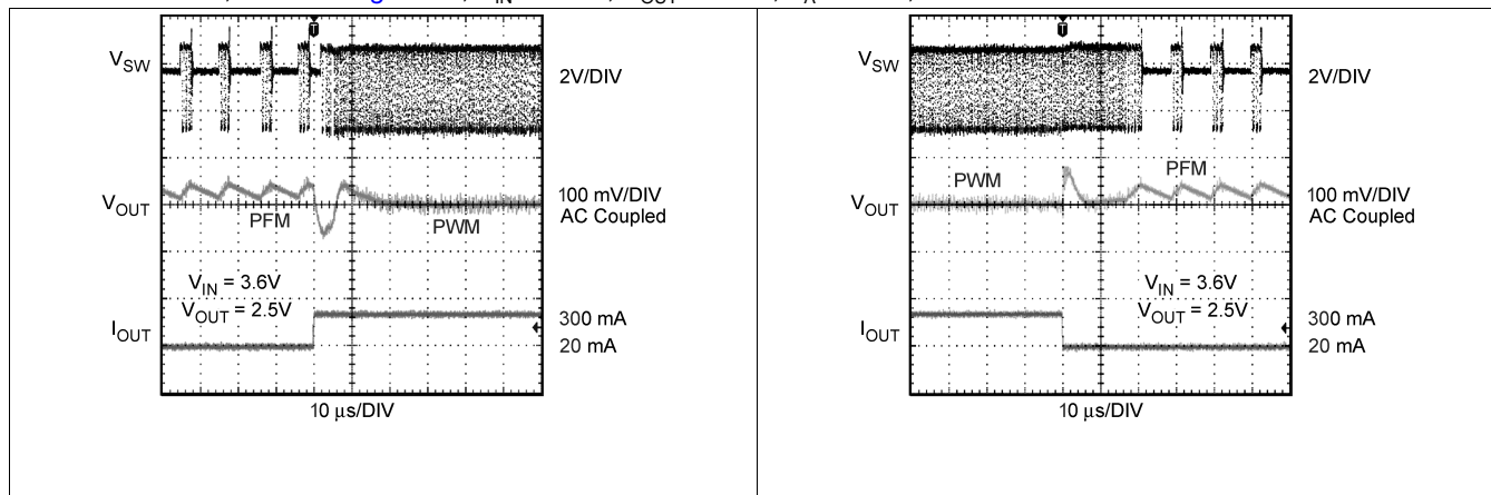
Figure 25. PFM-to-PWM Mode Change by Load Transients
