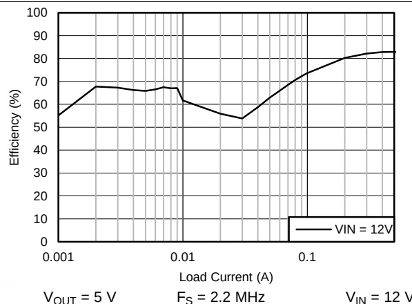
Figure 78. Efficiency
