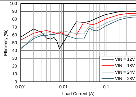
Figure 2. Efficiency
