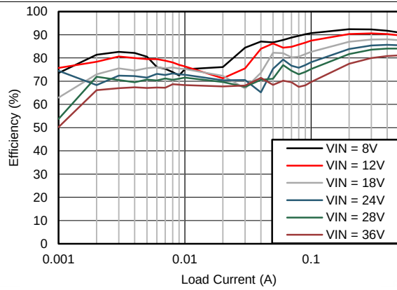
Figure 1. Efficiency
