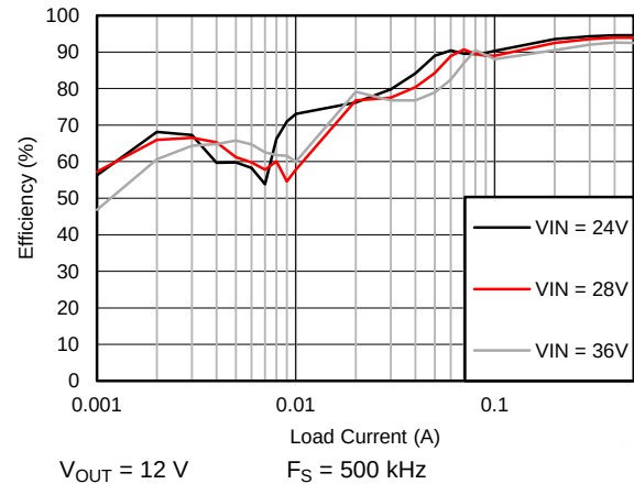
Figure 84. Efficiency
