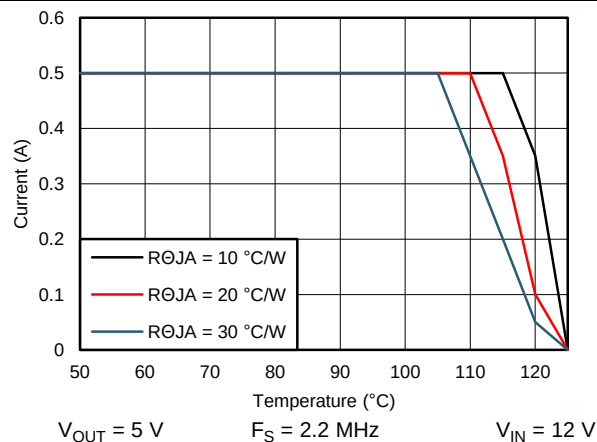
Figure 82. Derating Curve
