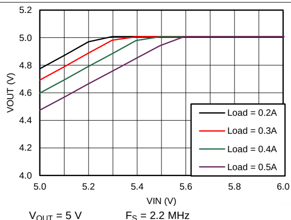
Figure 80. Dropout Curve
