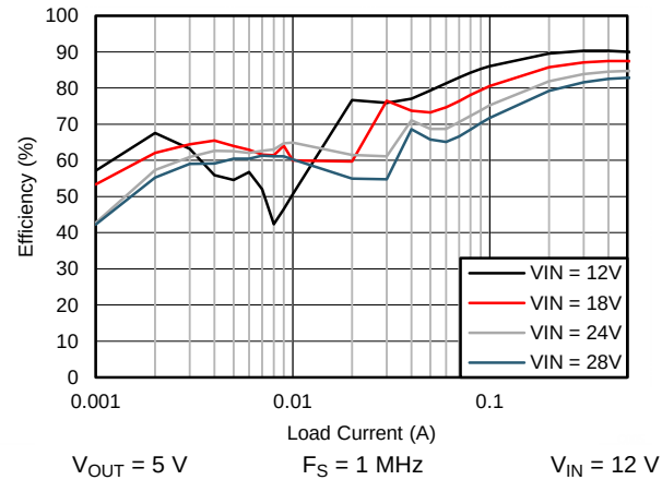
Figure 72. Efficiency
