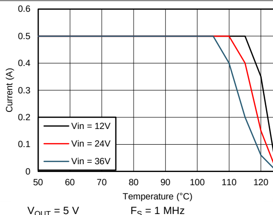
Figure 92. Derating Curve with R_{\theta JA} = 20^\circ\text{C/W}
