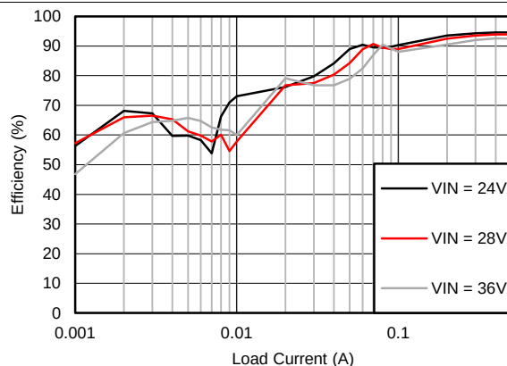
Figure 3. Efficiency
