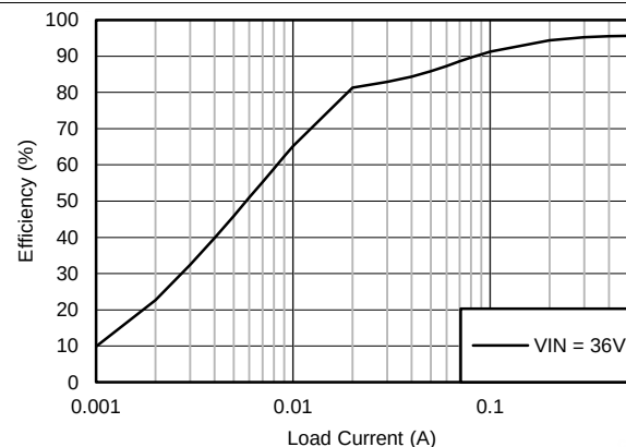
Figure 4. Efficiency
