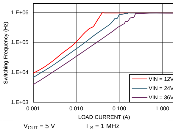
Figure 94. Switching Frequency vs I_{OUT} in PFM Operation
