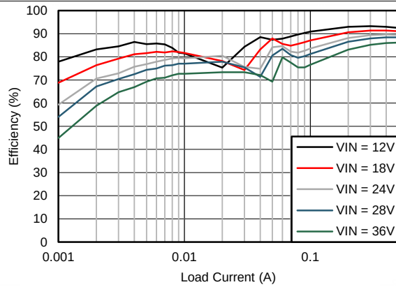
Figure 1. Efficiency
