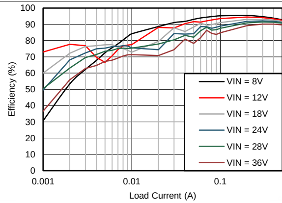
Figure 2. Efficiency
