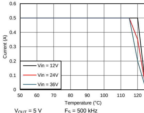
Figure 90. Derating Curve with R_{\theta JA} = 20^\circ\text{C/W}
