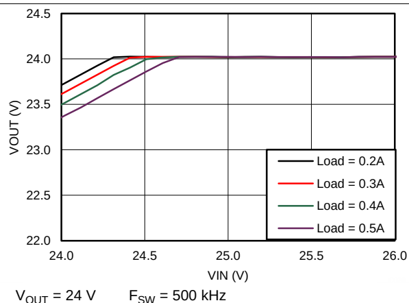
Figure 18. Dropout Curve
