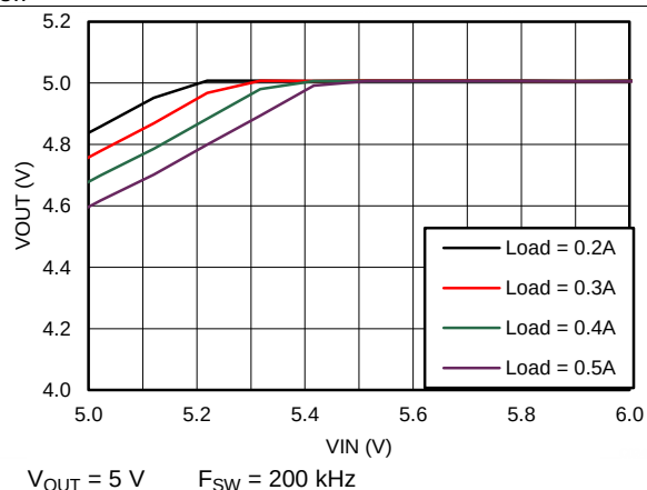
Figure 14. Dropout Curve
