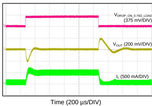
Figure 75. Load Transient Between 0.05 A and 0.5 A
