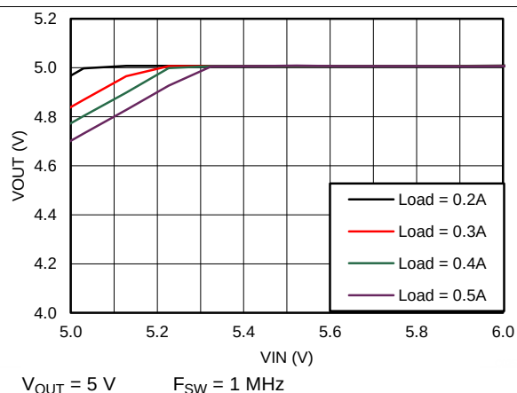
Figure 16. Dropout Curve
