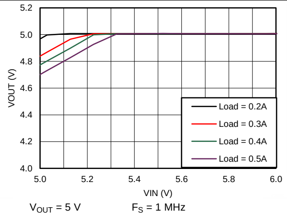
Figure 74. Dropout Curve
