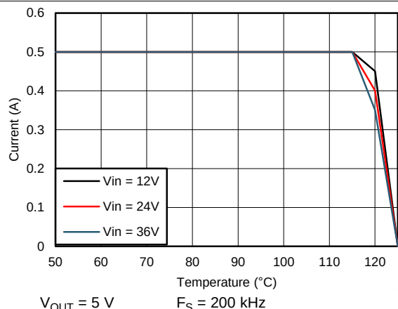
Figure 91. Derating Curve with R_{\theta JA} = 20^\circ\text{C/W}
