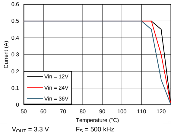
Figure 89. Derating Curve with R_{\theta JA} = 20^\circ\text{C/W}
