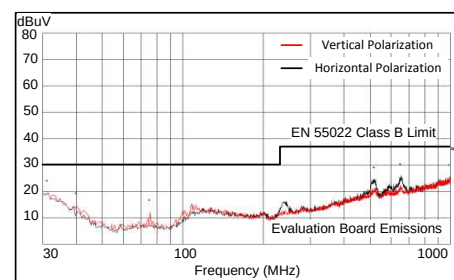
Radiated Emission Graph with V_{IN} = 12 V, V_{OUT} = 3.3 V, F_{SW} = 500 kHz, I_{OUT} = 0.5 A
