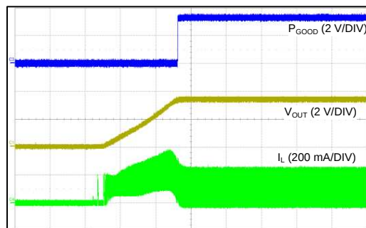
Figure 98. Start-up Into Full Load With Internal Soft-Start Rate
