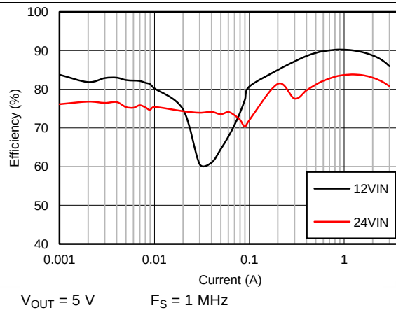
Figure 4. Efficiency
