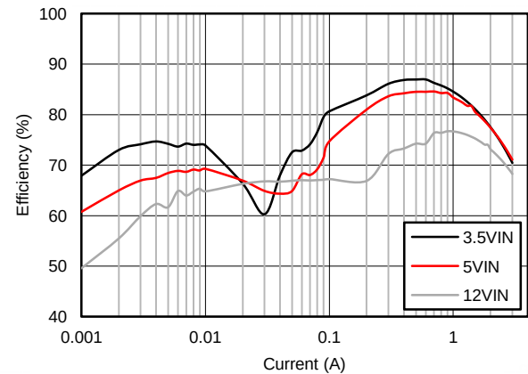
Figure 50. Efficiency
