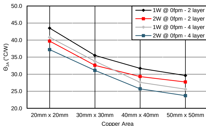
Figure 98. R_{JA} vs Copper Area 2 oz Copper on Outer Layers and 1 oz Copper on Inner Layers
