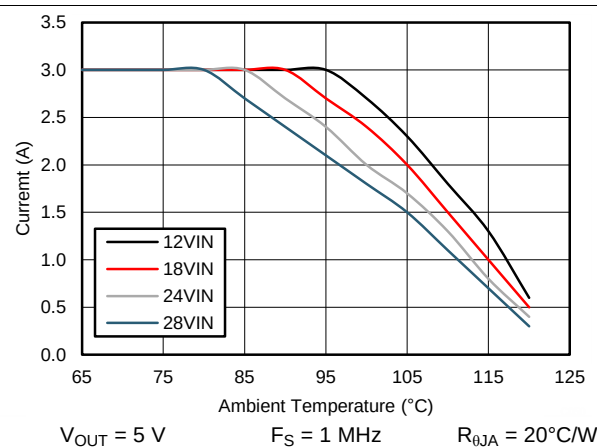
Figure 84. Derating Curve
