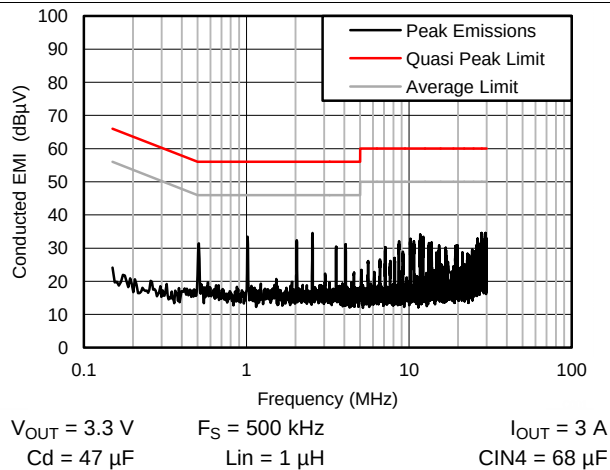
Figure 33. Conducted EMI Curve
