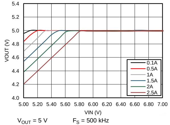
Figure 76. Dropout Curve
