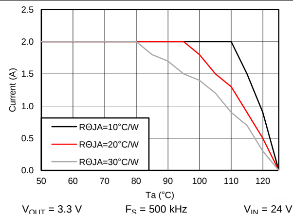
Figure 52. Derating Curve
