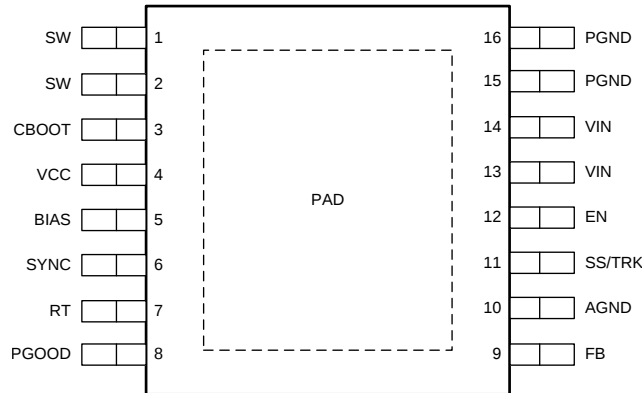
PWP Package 16-Pin HTSSOP With PowerPAD™ Top View
