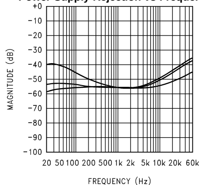
Figure 28. V_{DD} = 12\text{V} , R_L = 8\Omega , SE operation, V_{\text{RIPPLE}} = 200\text{mV}_{\text{p-p}} , A_V = 10 , at (from top to bottom at 60Hz): C_{\text{BYPASS}} = 1\mu\text{F} , C_{\text{BYPASS}} = 4.7\mu\text{F} , C_{\text{BYPASS}} = 10\mu\text{F}
