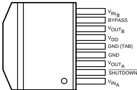
Figure 2. Plastic Package, DDPK Top View See Package Number KTW0009A
