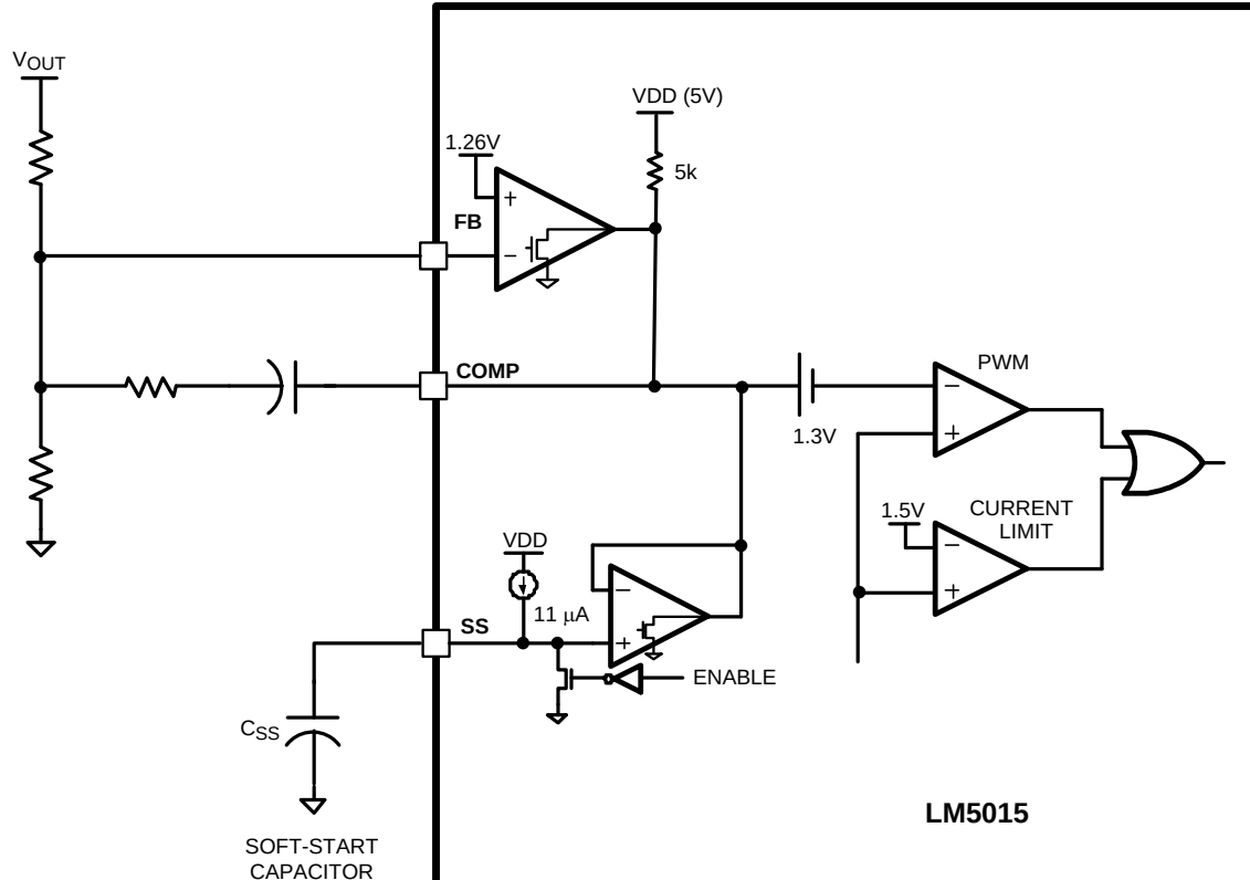
Figure 20. Soft-Start
