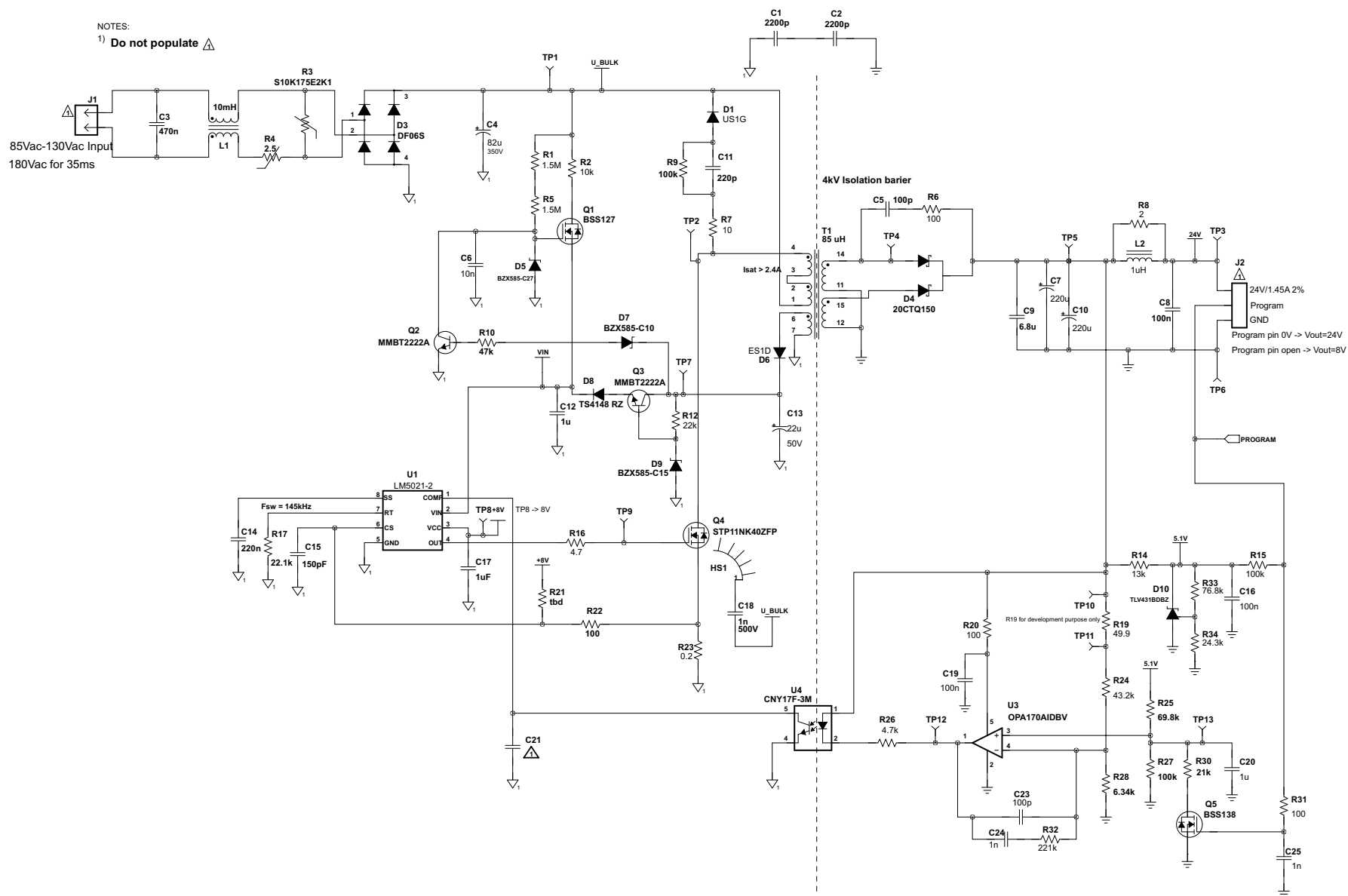
Figure 14. Typical Application Circuit
