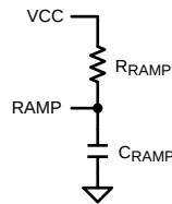
Figure 15. R_{RAMP} to VCC for V_{OUT} > 7.5\text{ V}
