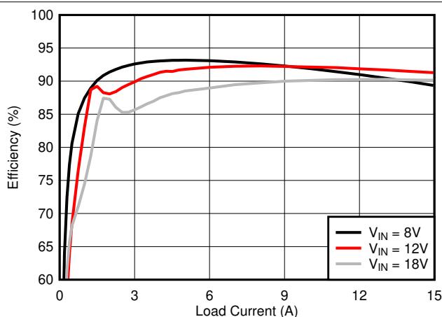
Figure 10-22. Efficiency Versus I_{OUT} , 5-V Output
