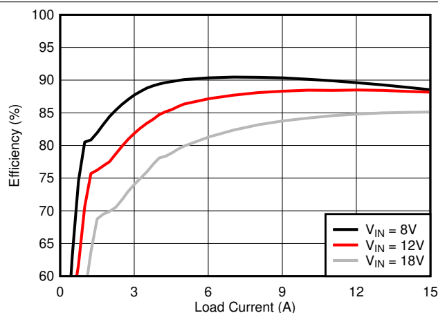
Figure 10-23. Efficiency Versus I_{OUT} , 3.3-V Output
