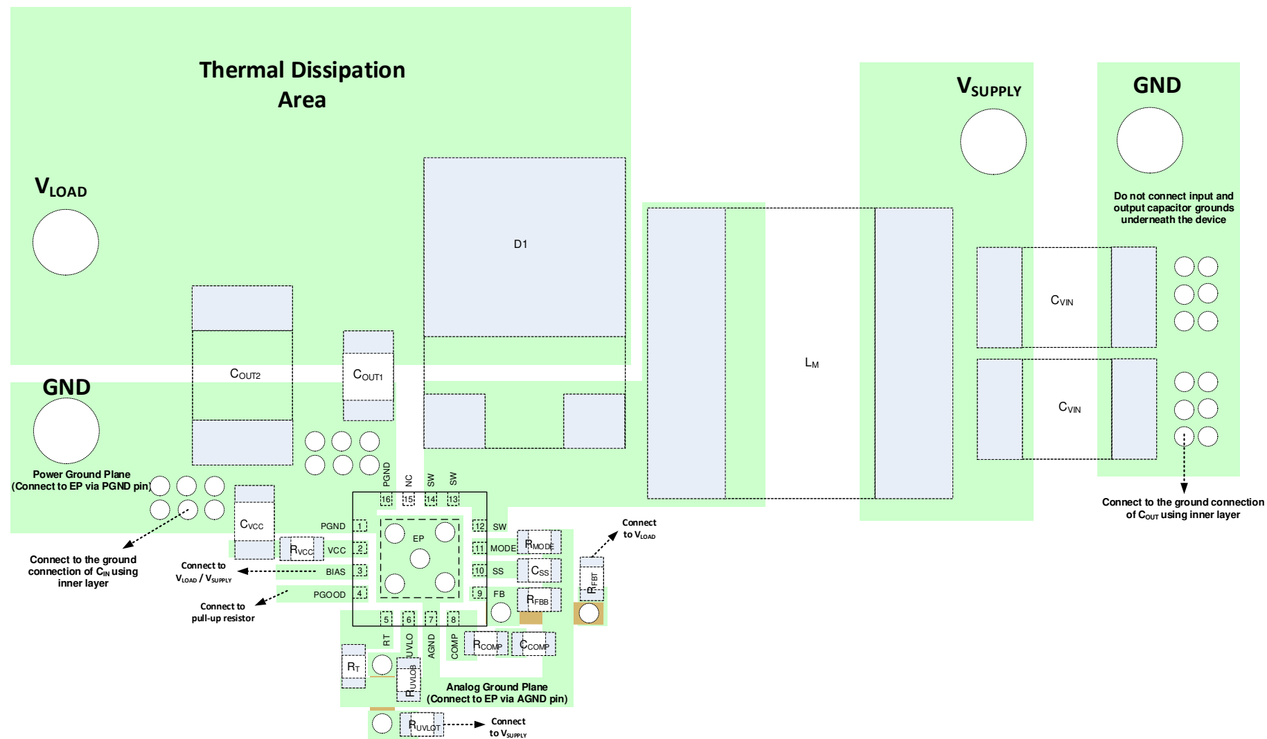
Figure 11-1. PCB Layout Example
