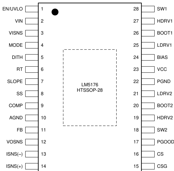
Figure 5-1. HTSSOP-28 PWP Package Top View
