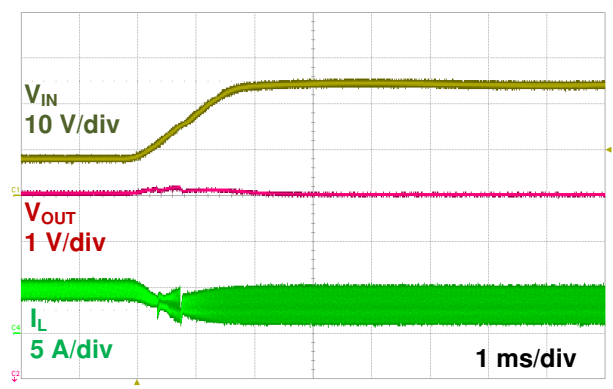
Figure 8-5. Line Transient Response (8 V - 24 V, I_{OUT} = 2 \text{ A} )
