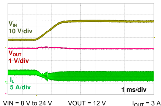
Figure 6-18. Line Transient
