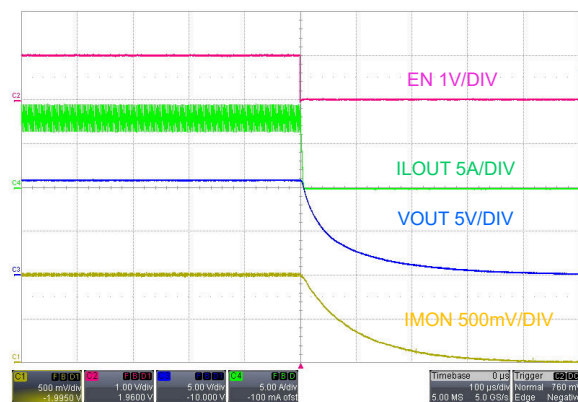
Figure 7-8. Shutdown, EN OFF, V SUPPLY = 48V, I LOAD = 8A Resistive Load
