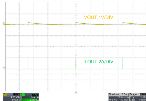
Figure 7-10. No Load Operation in PFM Mode, V SUPPLY = 48V, I LOAD = 0A
