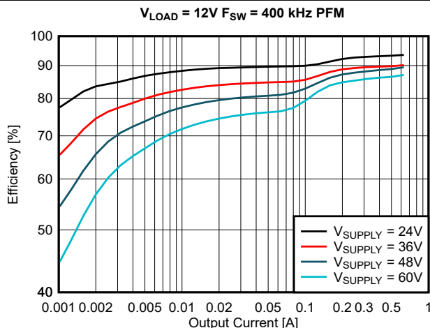
Figure 7-6. PFM Mode Efficiency, Log Scale
