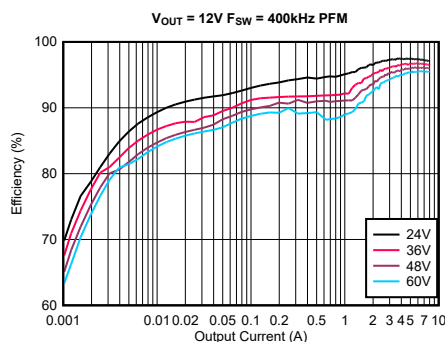
LM5192-Q1 Efficiency
