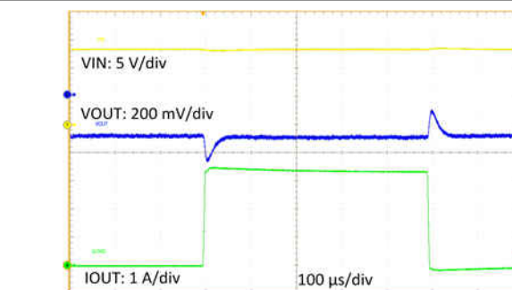
Figure 9-38. Load Transient
