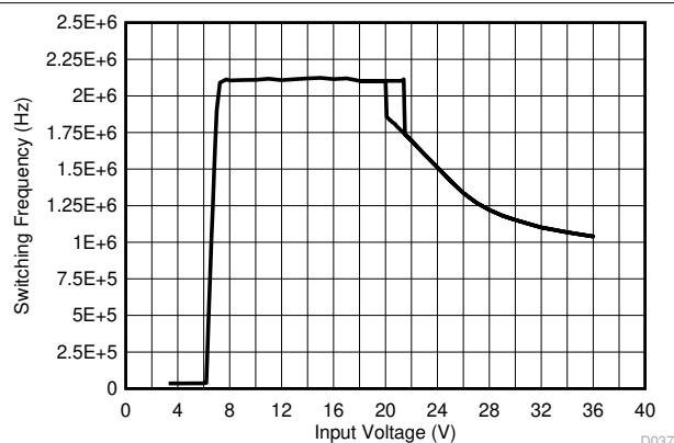
Figure 9-35. Switching Frequency vs Input Voltage
