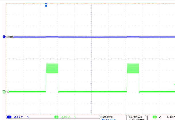
Figure 9-34. LM61430-Q1 Short Circuit Protection
