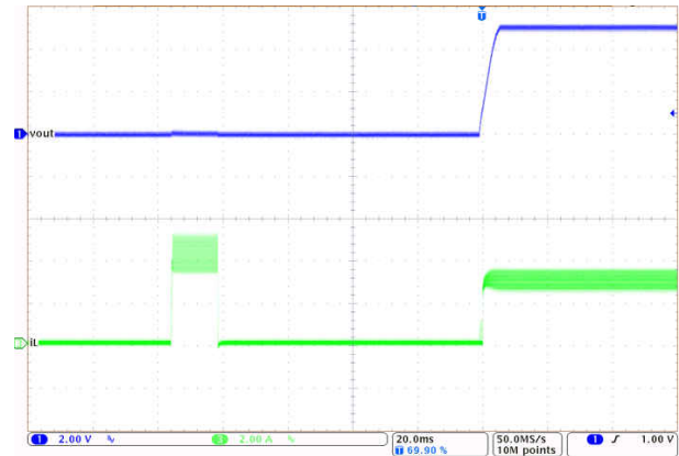
Figure 8-13. Short-Circuit Recovery
