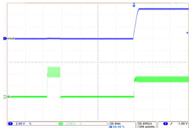
Figure 9-35. LM61430-Q1 Short Circuit Recovery
