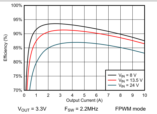
Figure 8-10. Efficiency
