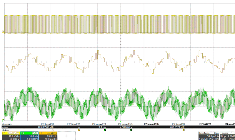
Figure 7-11. Output Ripple Without Ripple Cancellation Showing V_{\text{SW}} (Top), F_{\text{SW}} (Middle), V_{\text{OUT}} (Bottom)
