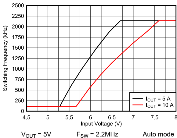
Figure 8-25. Frequency Dropout
