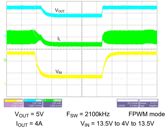
Figure 8-34. Recovery from Dropout
