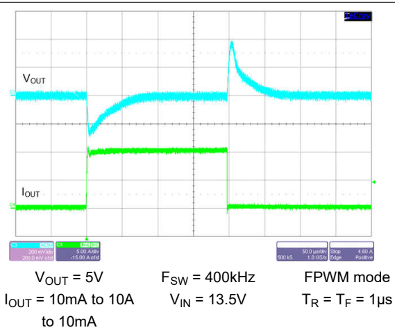
Figure 8-36. Load Transient
