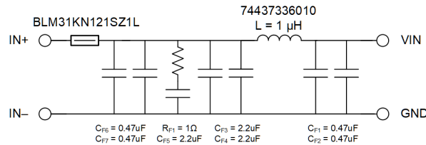
Figure 8-55. Recommended Input EMI Filter
