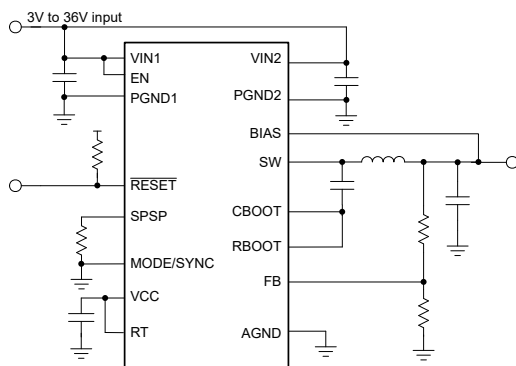
Simplified Schematic
