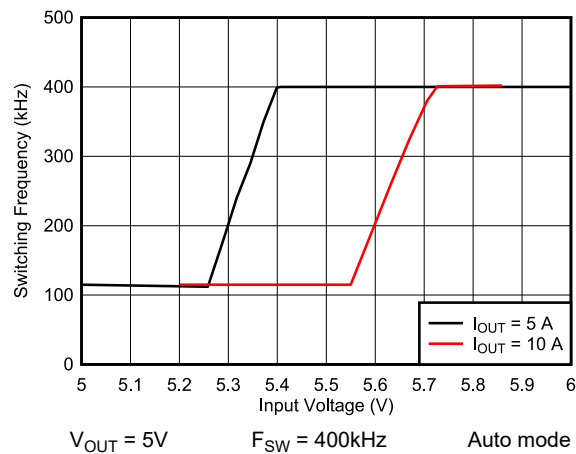
Figure 8-23. Frequency Dropout
