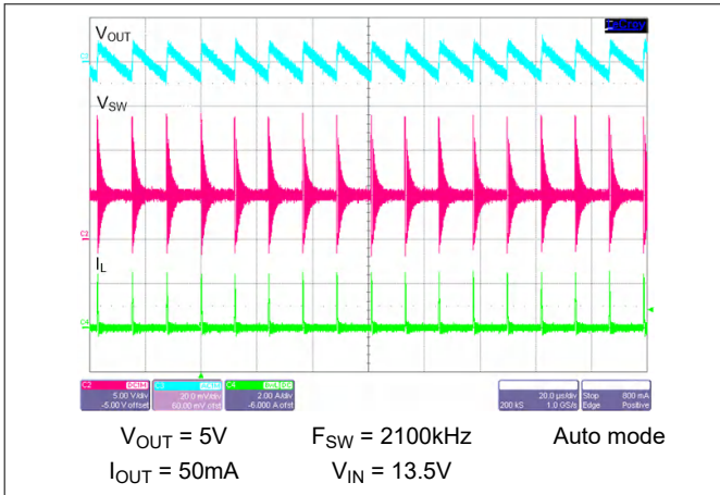
Figure 8-27. Switching Waveform and V_{OUT} Ripple
