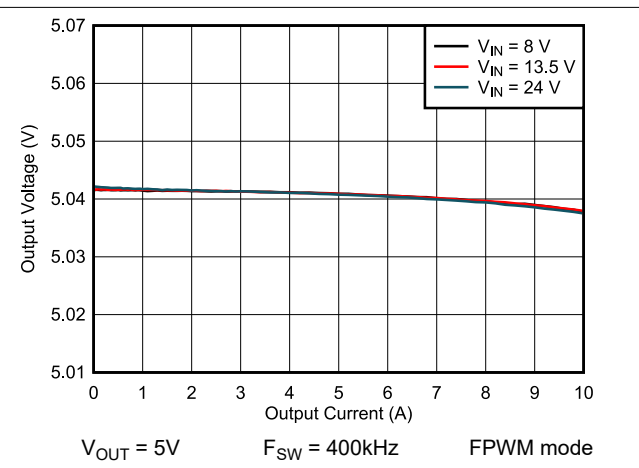
Figure 8-12. Load and Line Regulation
