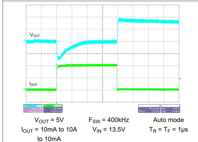
Figure 8-35. Load Transient
