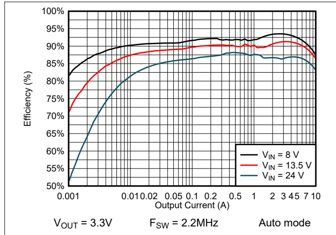
Figure 8-9. Efficiency
