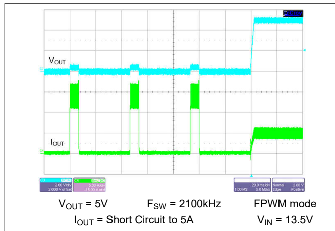
Figure 8-33. Short-Circuit Recovery
