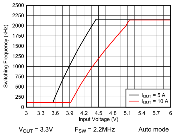
Figure 8-26. Frequency Dropout
