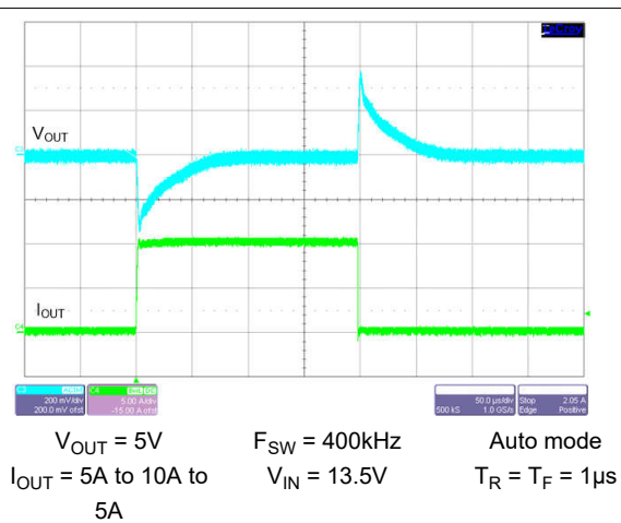
Figure 8-38. Load Transient
