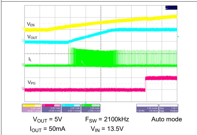
Figure 8-29. Start-Up With 50mA Load
