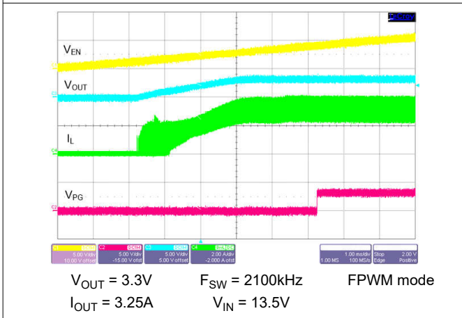
Figure 8-31. Start-Up With 3.25A Load
