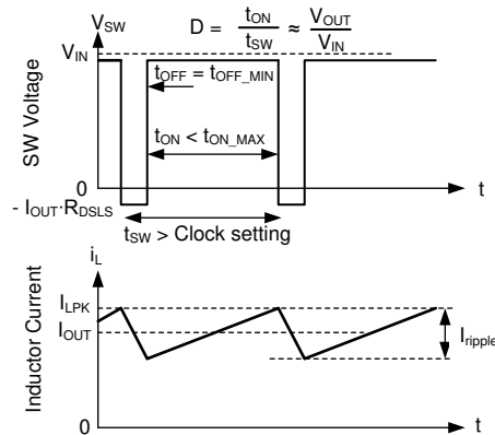
Figure 7-24. Frequency and Output Voltage in Dropout
