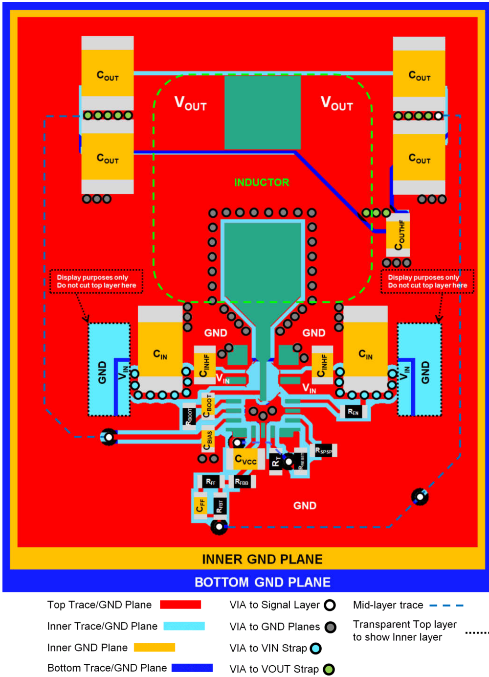
Figure 8-57. Layout Example
