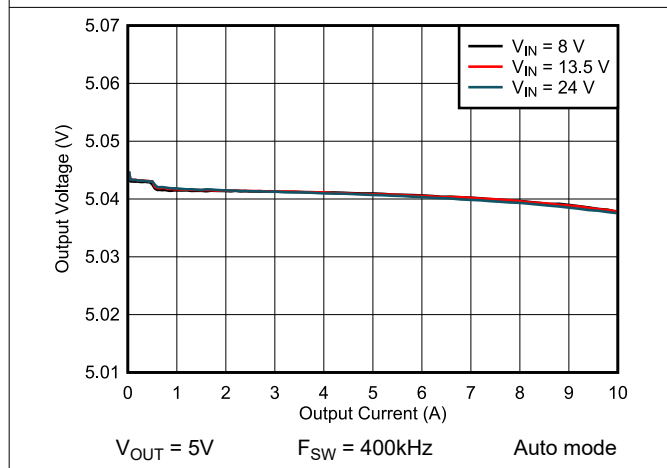
Figure 8-11. Load and Line Regulation
