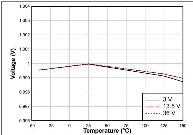
Figure 6-1. Feedback Voltage
