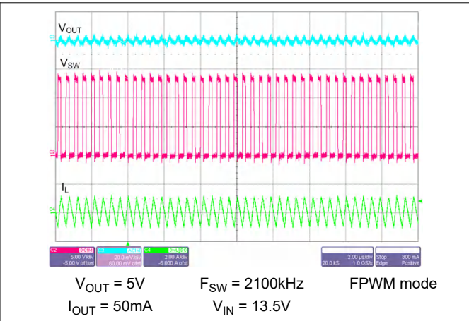
Figure 8-28. Switching Waveform and V_{OUT} Ripple
