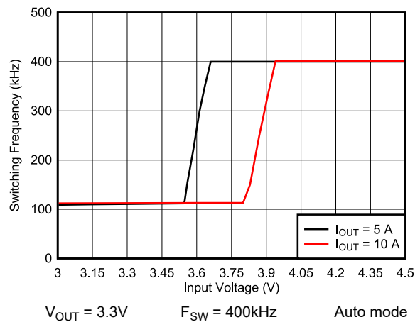
Figure 8-24. Frequency Dropout
