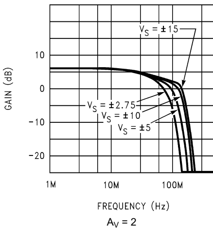
Figure 5-93. Closed-Loop Frequency Response vs Supply Voltage
