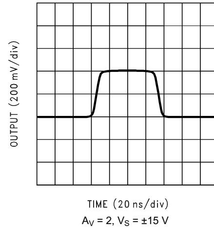
Figure 5-90. Small-Signal Pulse Response
