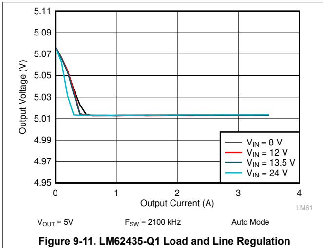
Figure 9-11. LM62435-Q1 Load and Line Regulation
