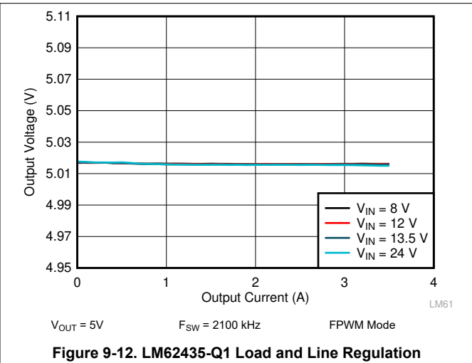
Figure 9-12. LM62435-Q1 Load and Line Regulation
