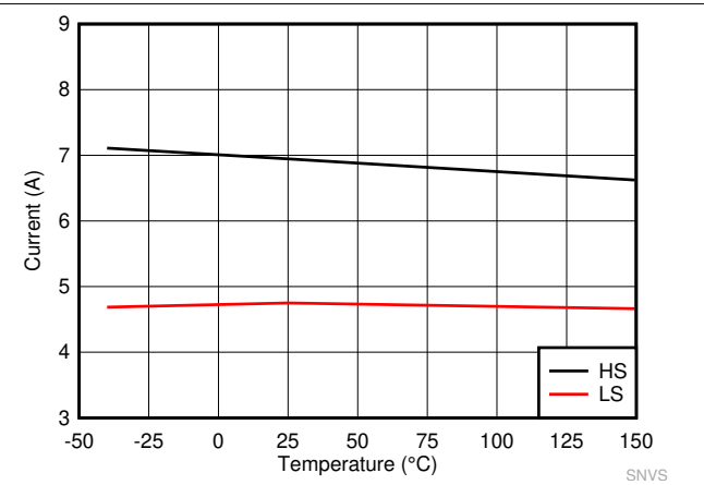
Figure 7-4. LM62435-Q1 High-side and Low-side Current Limits
