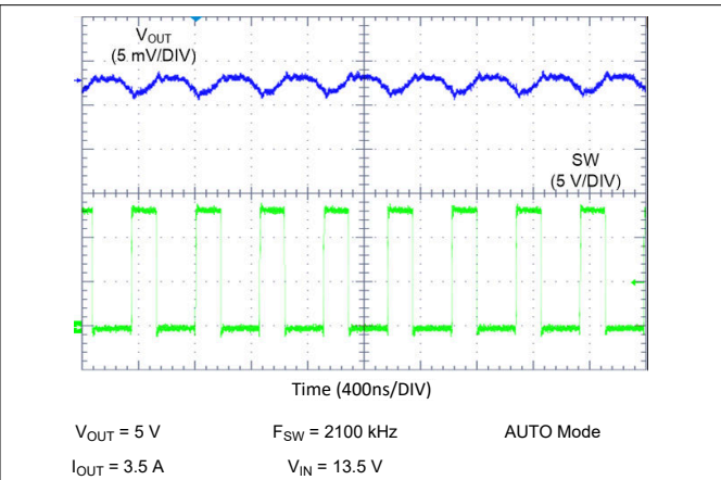
Figure 9-18. LM62435-Q1 Switching Waveform and V_{OUT} Ripple
