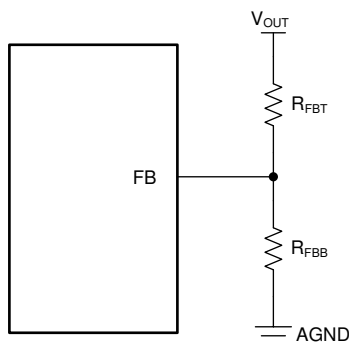
Figure 8-17. Setting Output Voltage of Adjustable Versions
