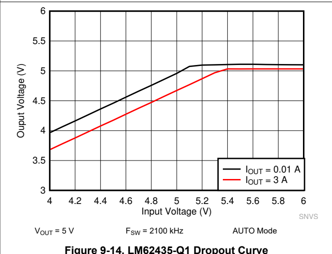
Figure 9-14. LM62435-Q1 Dropout Curve
