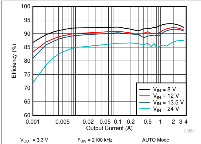
Figure 9-5. LM62435-Q1 Efficiency
