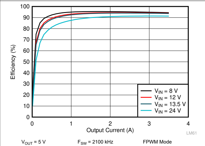
Figure 9-8. LM62435-Q1 Efficiency
