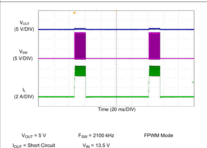
Figure 9-22. LM62435-Q1 Short Circuit Performance
