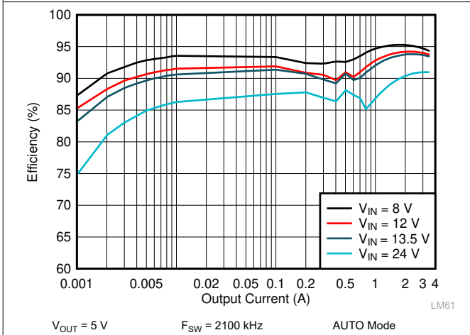
Figure 9-7. LM62435-Q1 Efficiency
