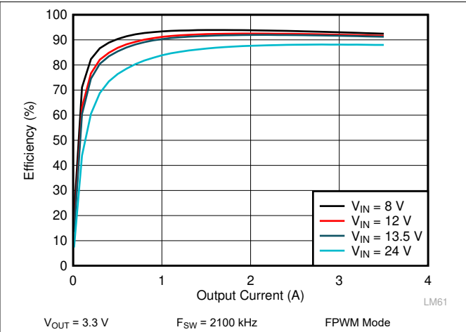
Figure 9-6. LM62435-Q1 Efficiency
