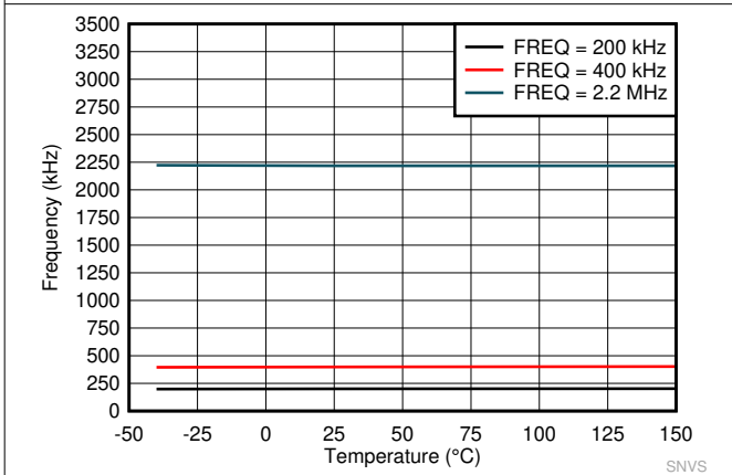
Figure 7-5. Switching Frequency Set by SYNC
