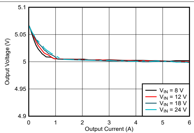
Figure 8-4. LM634x0-Q1 Load and Line Regulation
