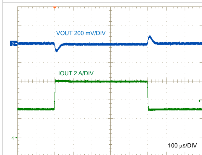
Figure 8-26. LM634x0-Q1 Load Transient, I_{OUT} = 3A to 6A
