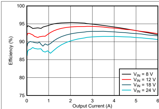
Figure 8-3. LM634x0-Q1 Efficiency
