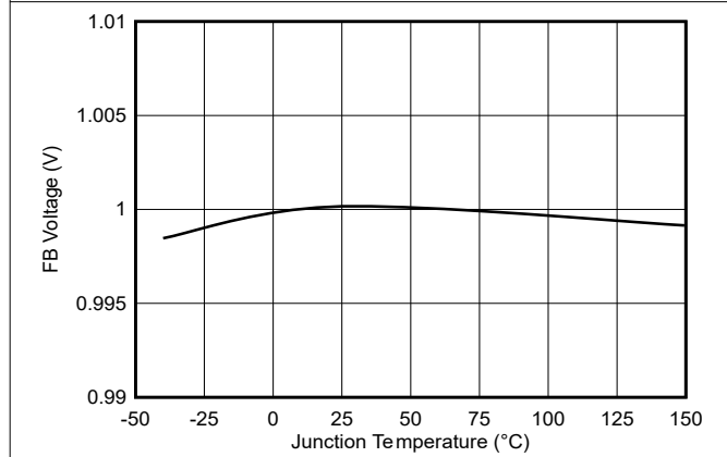
Figure 6-3. Feedback Voltage
