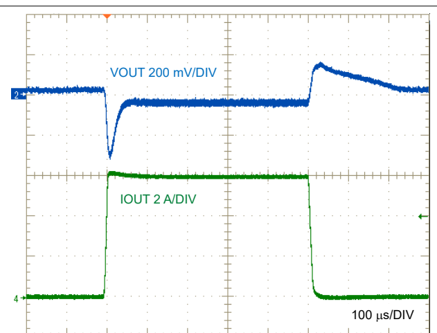
Figure 8-8. LM634x0-Q1 Load Transient, I_{OUT} = 0A to 6A
