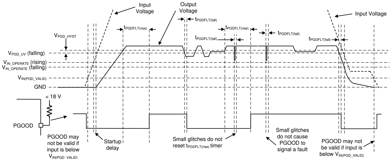
Figure 7-5. PGOOD Timing Diagram (Excludes OV Events)
