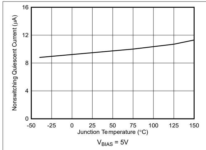
Figure 6-1. Non-Switching Input Supply Current
