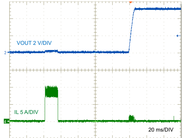
Figure 8-10. LM634x0-Q1 Short-Circuit Recovery to No Load
