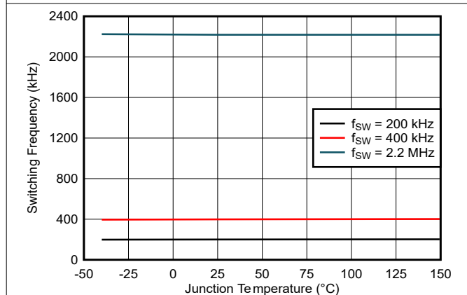
Figure 6-5. Switching Frequency Set by RT Resistor
