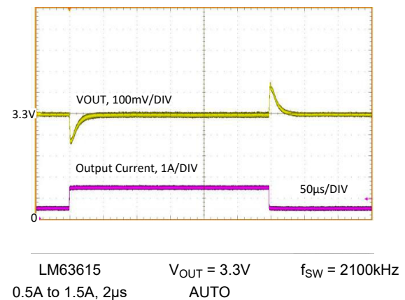
Figure 8-31. Load Transient
