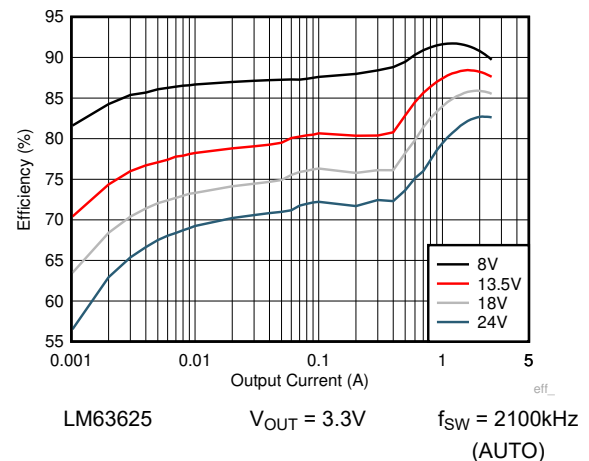
Figure 8-13. Efficiency
