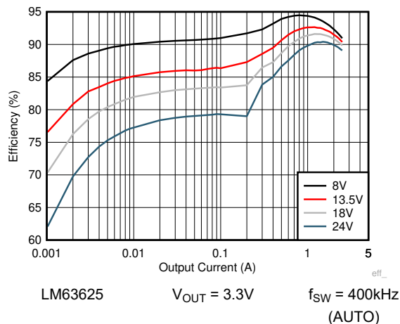
Figure 8-12. Efficiency
