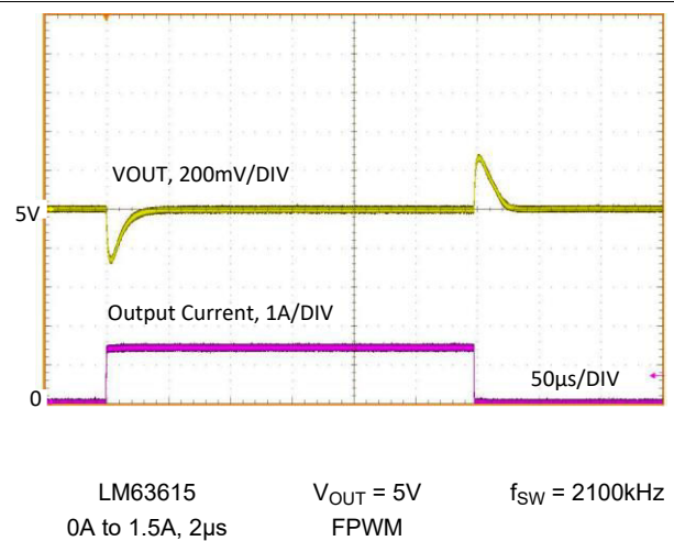
Figure 8-29. Load Transient
