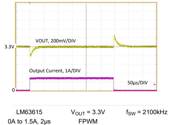
Figure 8-27. Load Transient
