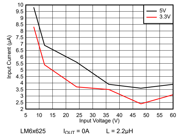
Figure 8-72. No Load Input Supply Current - Auto Mode
