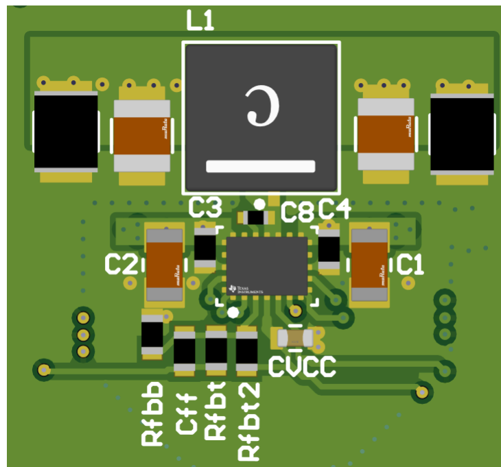
Figure 8-99. PCB Image
