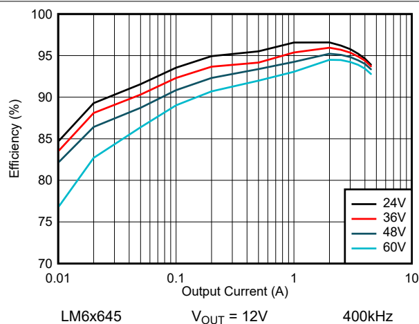
Figure 8-75. LM6x645 Efficiency - V_{OUT} = 12V - Auto Mode
