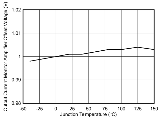
Figure 6-16. IMON Amplifier Voltage Offset vs Temperature
