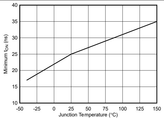
Figure 6-14. Minimum On-Time vs Temperature
