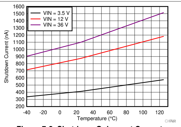
Figure 7-2. Shutdown Quiescent Current
