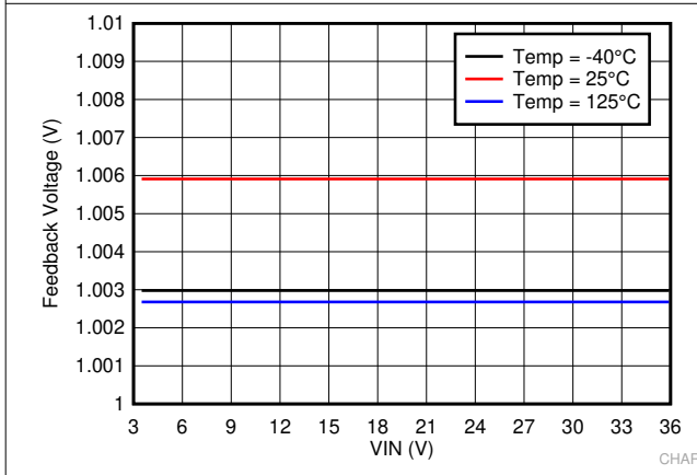
Figure 7-3. Feedback Voltage
