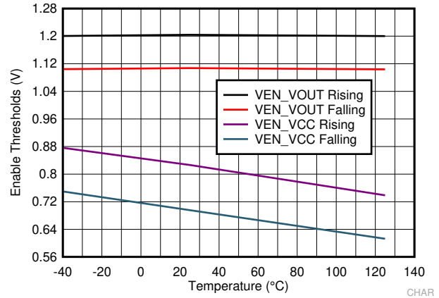
Figure 7-8. Enable Thresholds
