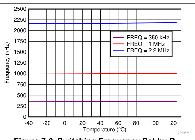
Figure 7-6. Switching Frequency Set by R_T Resistor
