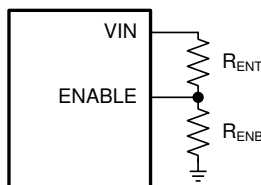
Figure 8-5. System UVLO
