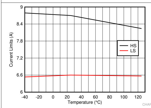
Figure 7-5. LM73605-Q1 High-Side and Low-Side Current Limit
