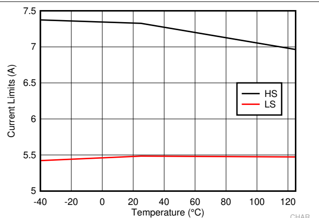
Figure 7-4. LM73605-Q1 High-Side and Low-Side Current Limits
