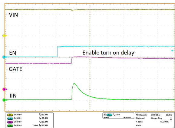
Figure 10-11. Enable Turn-ON Delay
