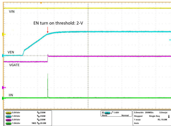
Figure 10-10. Enable Threshold
