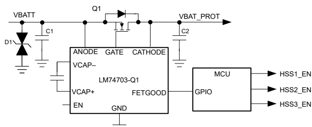
LM74703-Q1 Typical Application Schematic
