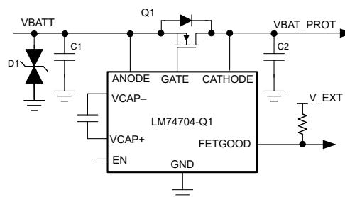
LM74704-Q1 Typical Application Schematic
