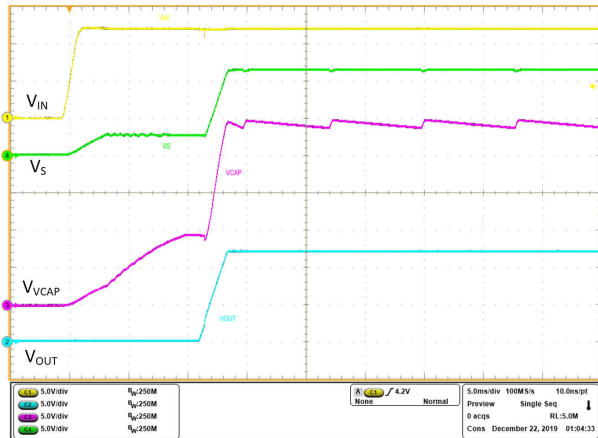
Figure 10-27. Power up 12 V - Charge Pump VCAP
