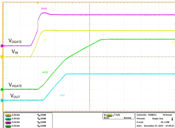
Figure 9-2. Startup 12 V with EN pulled to VIN
