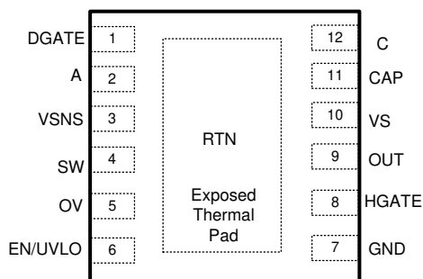
Figure 5-1. DRR Package, 12-Pin WSON (Top View)
