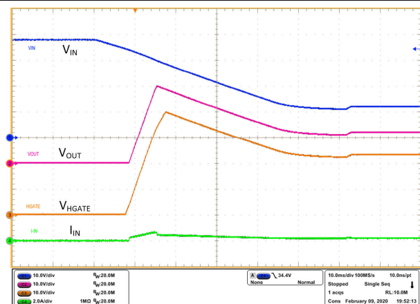
Figure 9-7. Overvoltage Recovery
