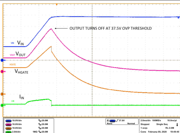
Figure 9-6. Overvoltage Cut-off
