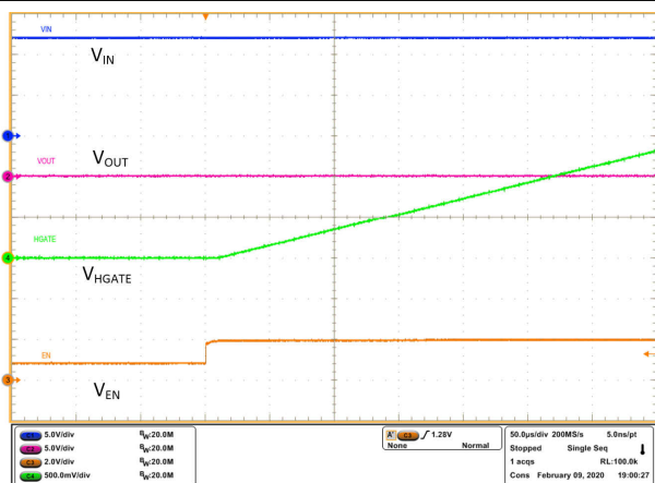
Figure 9-12. Enable Delay HGATE
