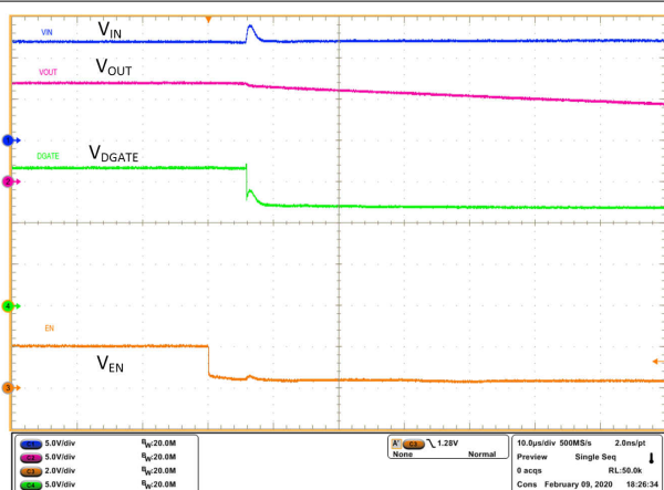
Figure 9-10. Disable Delay DGATE
