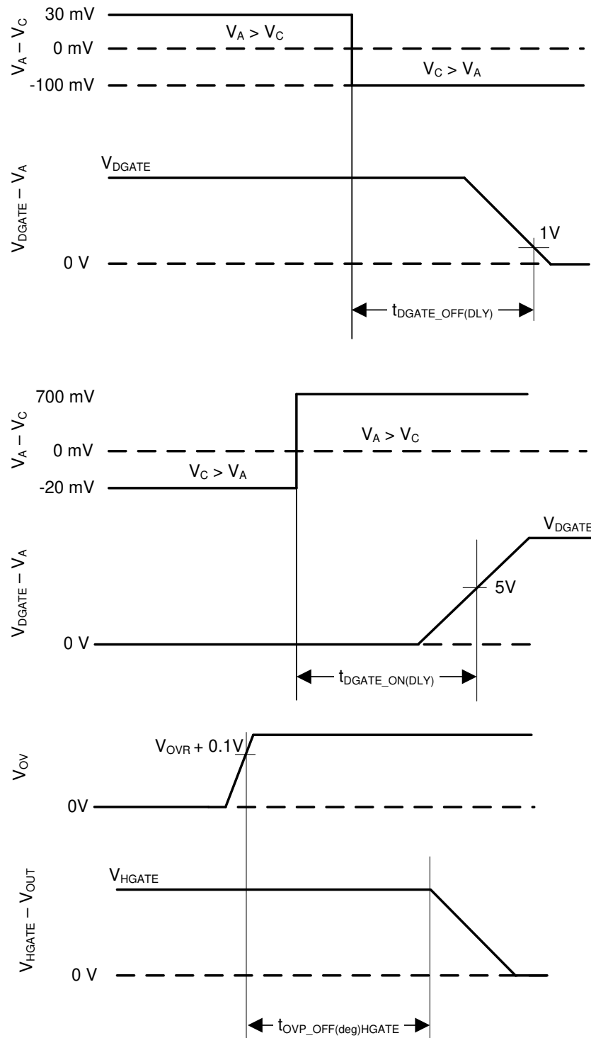
Figure 7-1. Timing Waveforms
