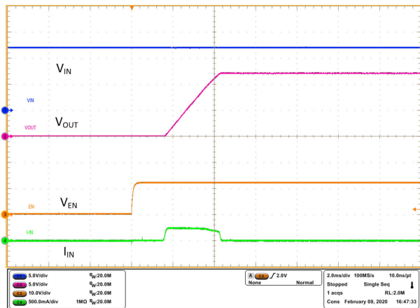
Figure 9-8. Turn ON with ENABLE Control
