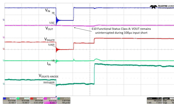
Figure 9-5. Input Micro-Short - LV124 E10 TC 2 100 \mu s
