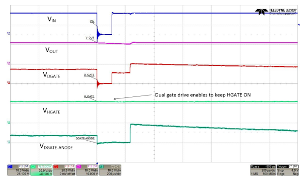
Figure 9-6. Input Micro-Short - LV124 E10 TC 2 100 \mu s with HGATE
