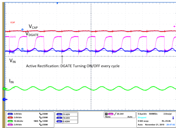
Figure 9-3. AC Super Imposed Test on 15 nC QGS- 2-V Peak-Peak 200 KHz
