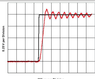
Figure 44. Pulse Response ( R_O = 4 \Omega , C_O = 1000 \text{ pF} , R_L = 2 \text{ k}\Omega )
