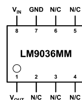
Figure 2. See Package Number DGK0008A Top View
