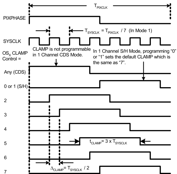
Figure 20. 1 Channel (Mode 1) CLAMP Timing
