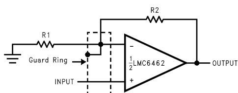
Figure 44. Non-Inverting Amplifier
