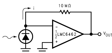
Figure 49. Photo Detector Circuit
