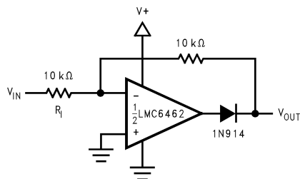
Figure 52. Full-Wave Rectifier with Input Current Protection ( R_I )
