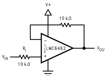
Figure 51. Half-Wave Rectifier with Input Current Protection ( R_i )
