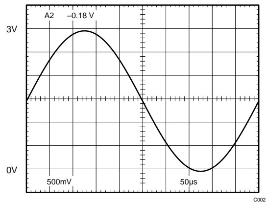
Rail-to-Rail Output
