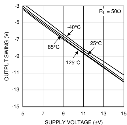
Figure 5-42. Negative Output Swing vs. Supply Voltage
