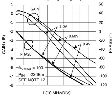
Frequency Response for Various V_G ( A_{VMAX} = 105 ) (Large Signal)
