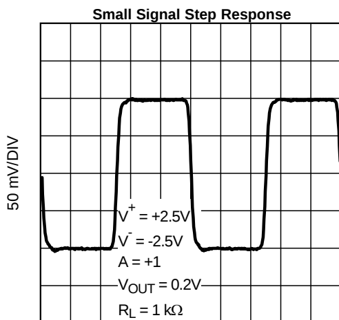
25 ns/DIV Figure 49.
