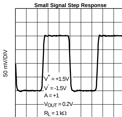
25 ns/DIV Figure 50.
