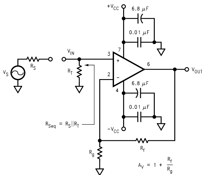
Figure 47. Non-Inverting Amplifier Configuration
