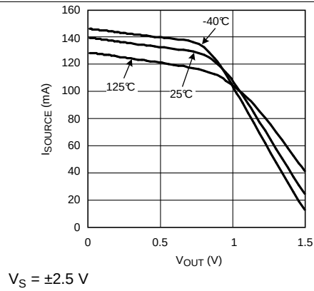
Figure 19. Sourcing Current vs. V_{OUT} (LMH6624)
