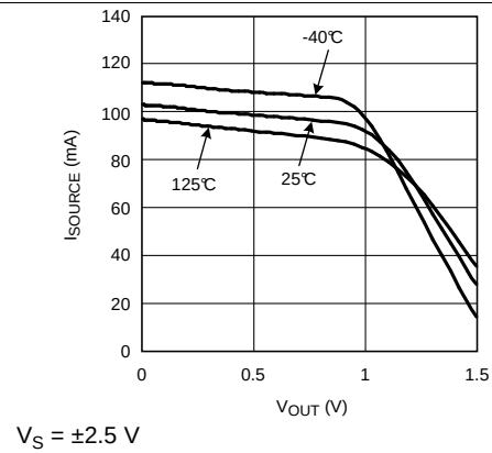
Figure 20. Sourcing Current vs. V_{OUT} (LMH6626)
