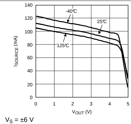
Figure 20. Sourcing Current vs. V_{OUT} (LMH6626)
