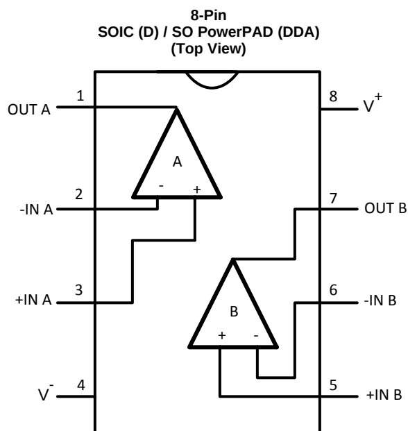
Pin Functions
