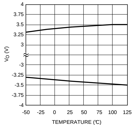
Figure 26. Voltage Swing vs Temperature
