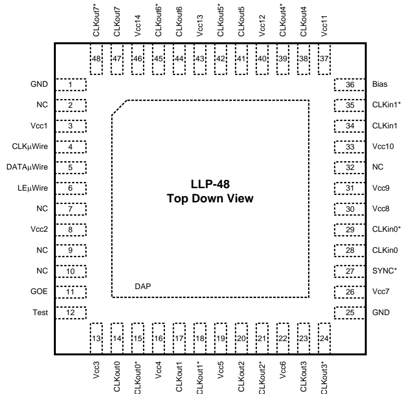
Figure 1. 48-Pin LLP Package
