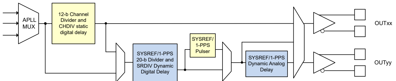
Figure 8-23. Programmable Static and Dynamic Output Delay
